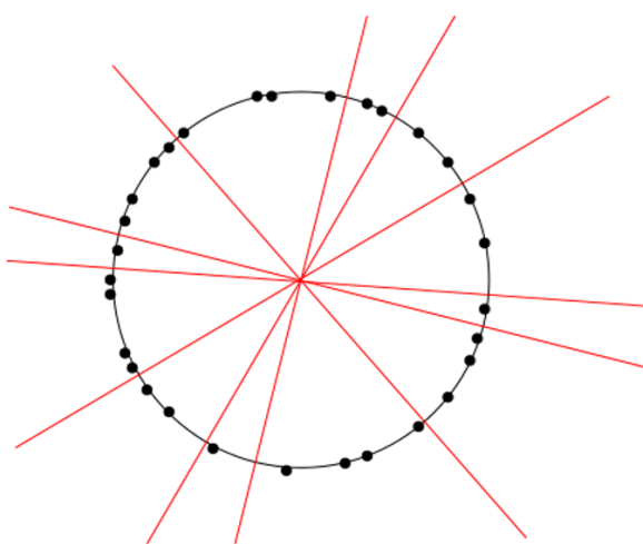
Figure 10.7: Nearby points on the circle generally lie on the same side of random lines through the origin. Locality-sensitive hash codes for each point can be composed as a sequence of sidedness tests (left or right) for any specific sequence of lines.
