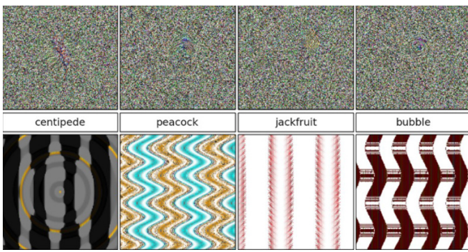
Figure 7.1: Synthetic images that are mistakenly recognized as objects by state-of-the-art Deep Learning neural networks, each with a confidence greater than 99.6%. Source: [NYC15].
